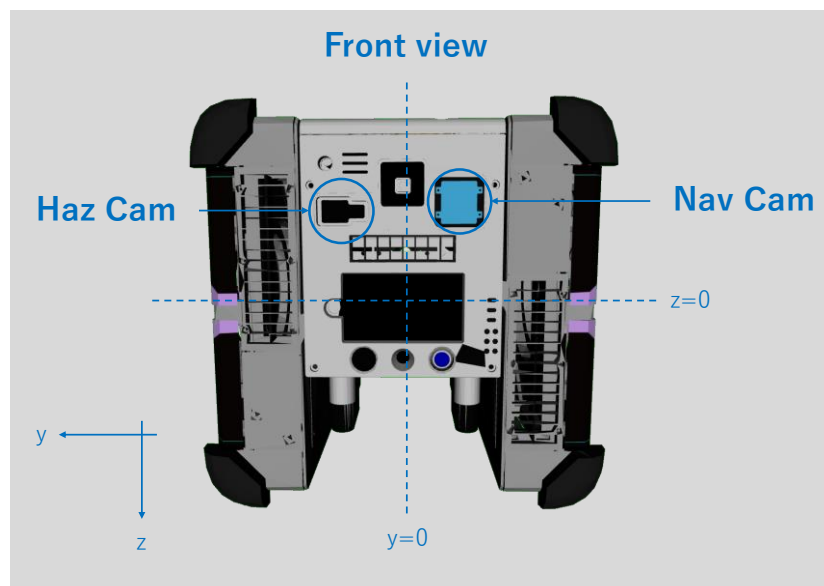
Figure 7-2 Astrobee Front View
