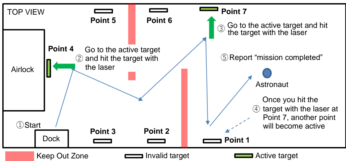
Figure 4.3-1 Game flow
